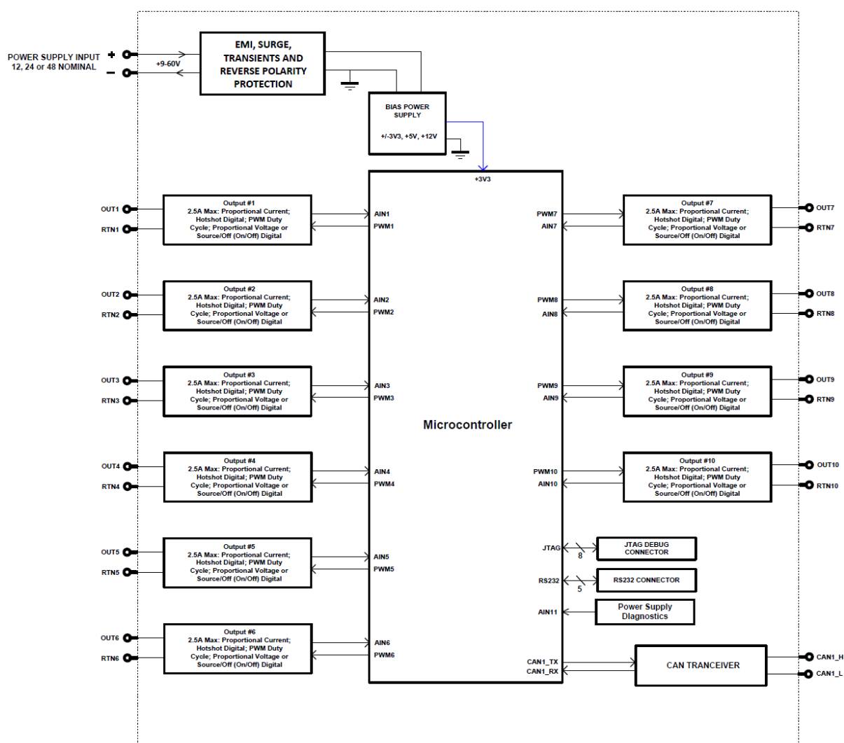
Figure 1 - Hardware Functional Block Diagram
