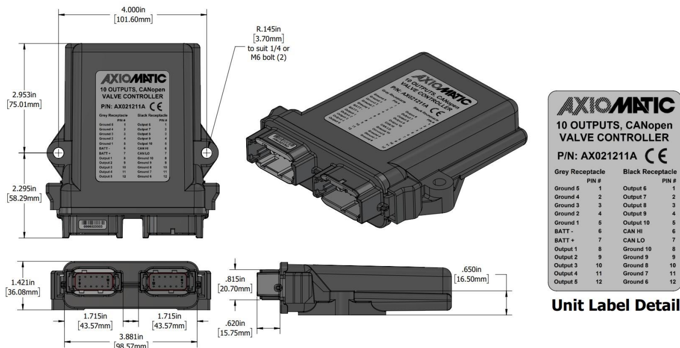
Figure 17 - Controller Dimensions
