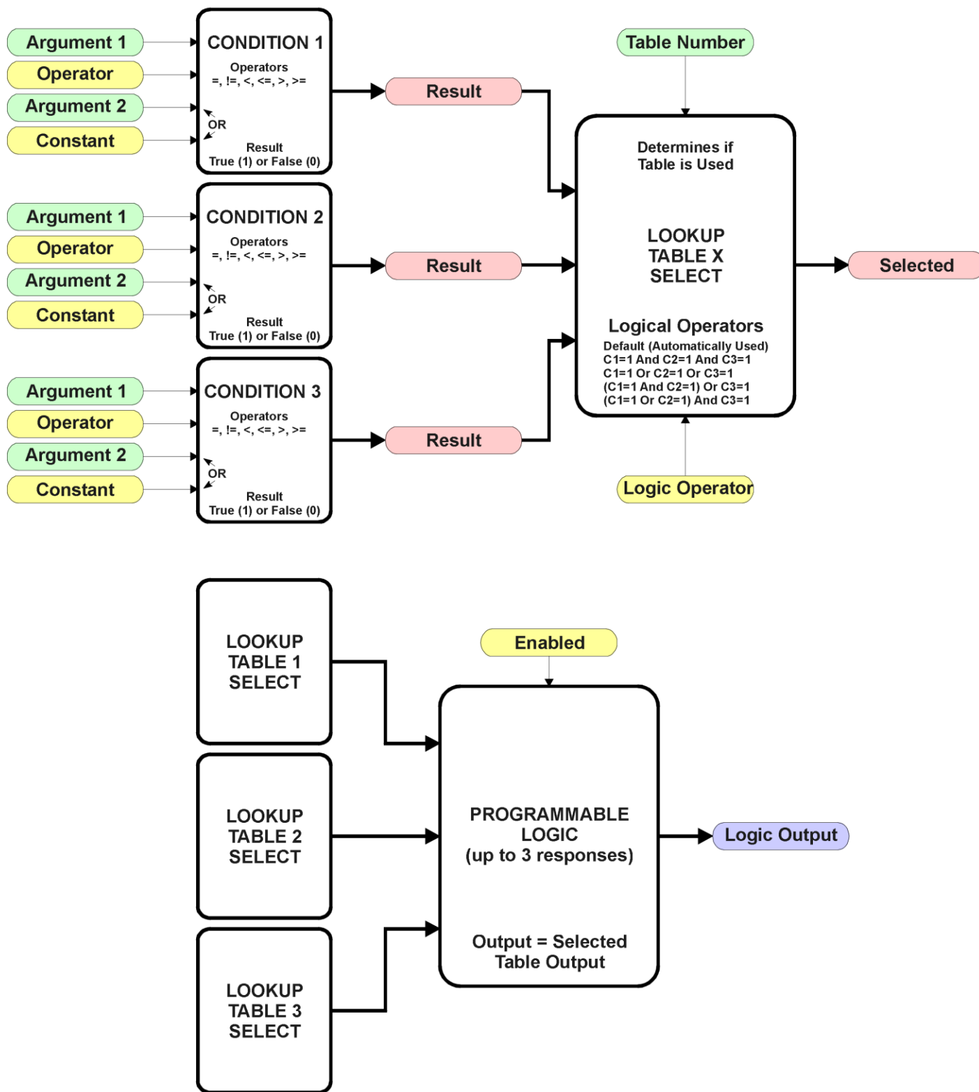
Figure 19 – Programmable Logic Function Block
