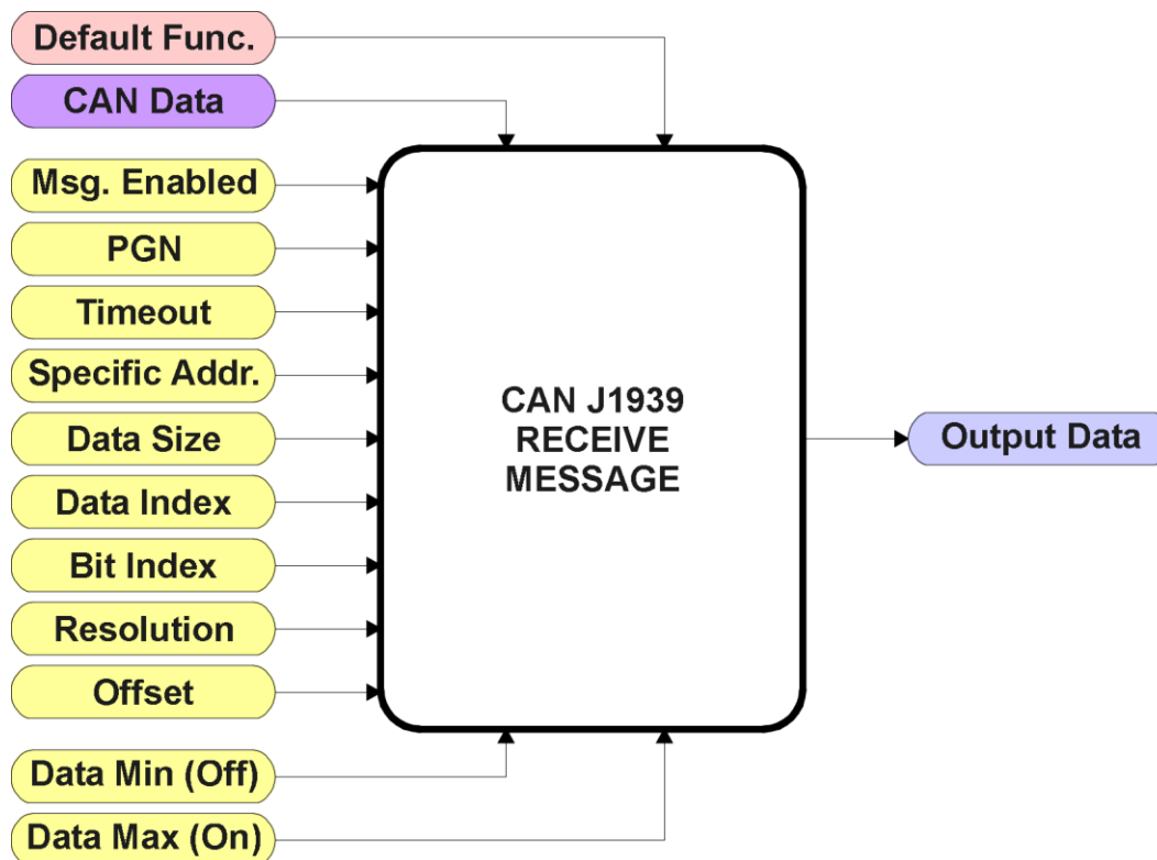
Figure 26 – CAN Receive Function Block
