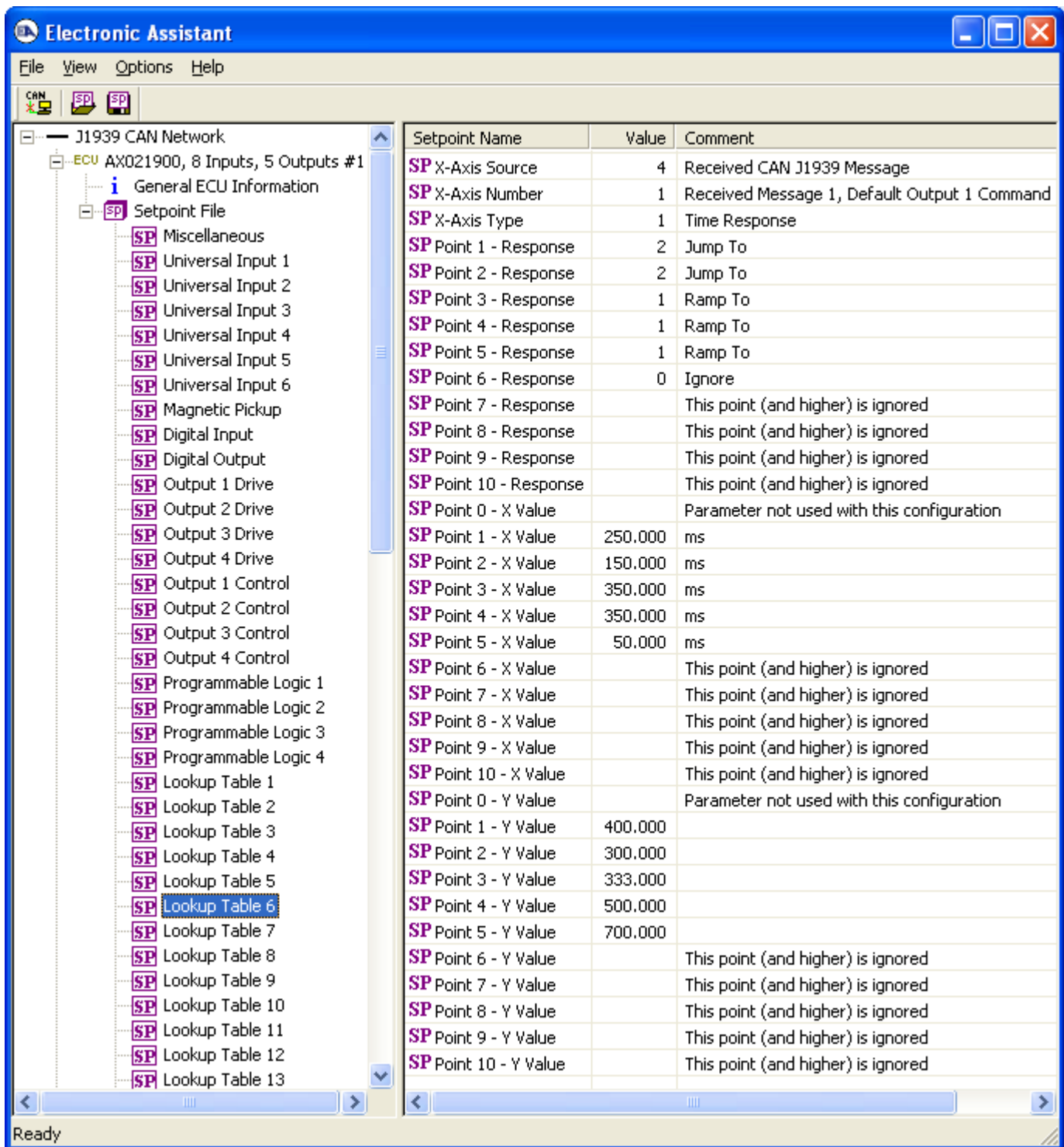
Figure 18 – Lookup Table “Soft Shift” Axiomatic EA Configuration
