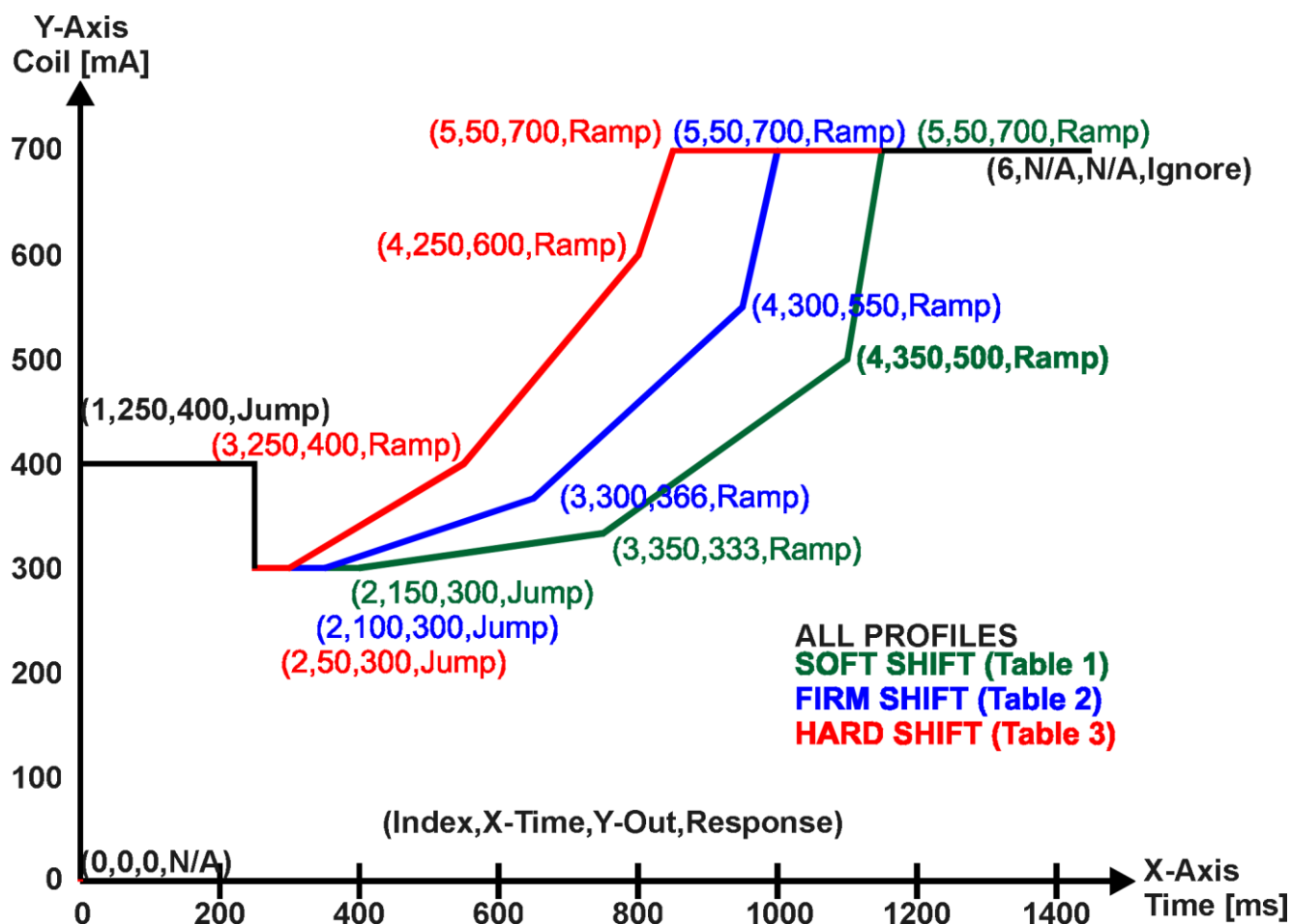
Figure 17 – Lookup Table Time Response Clutch Fill Profiles
