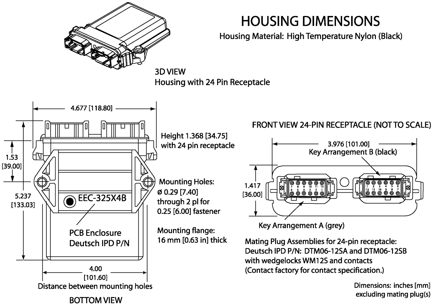
Figure 28 – Dimension Drawing
