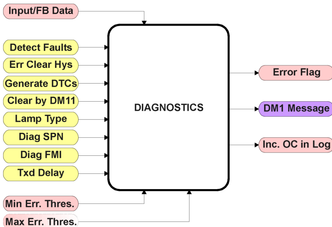
Figure 23 – Diagnostics Function Block
