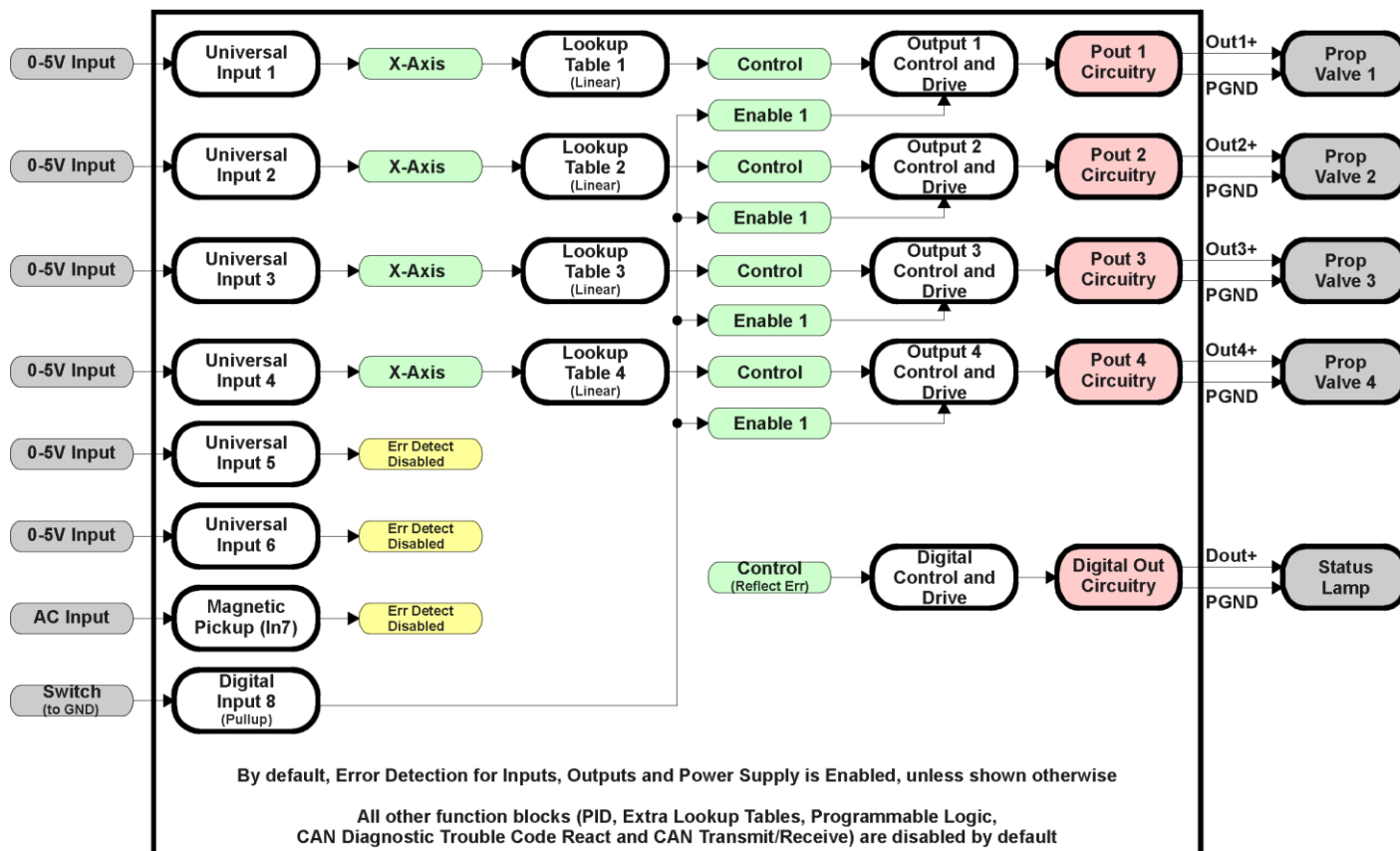
Figure 27 – Default Control Logic
