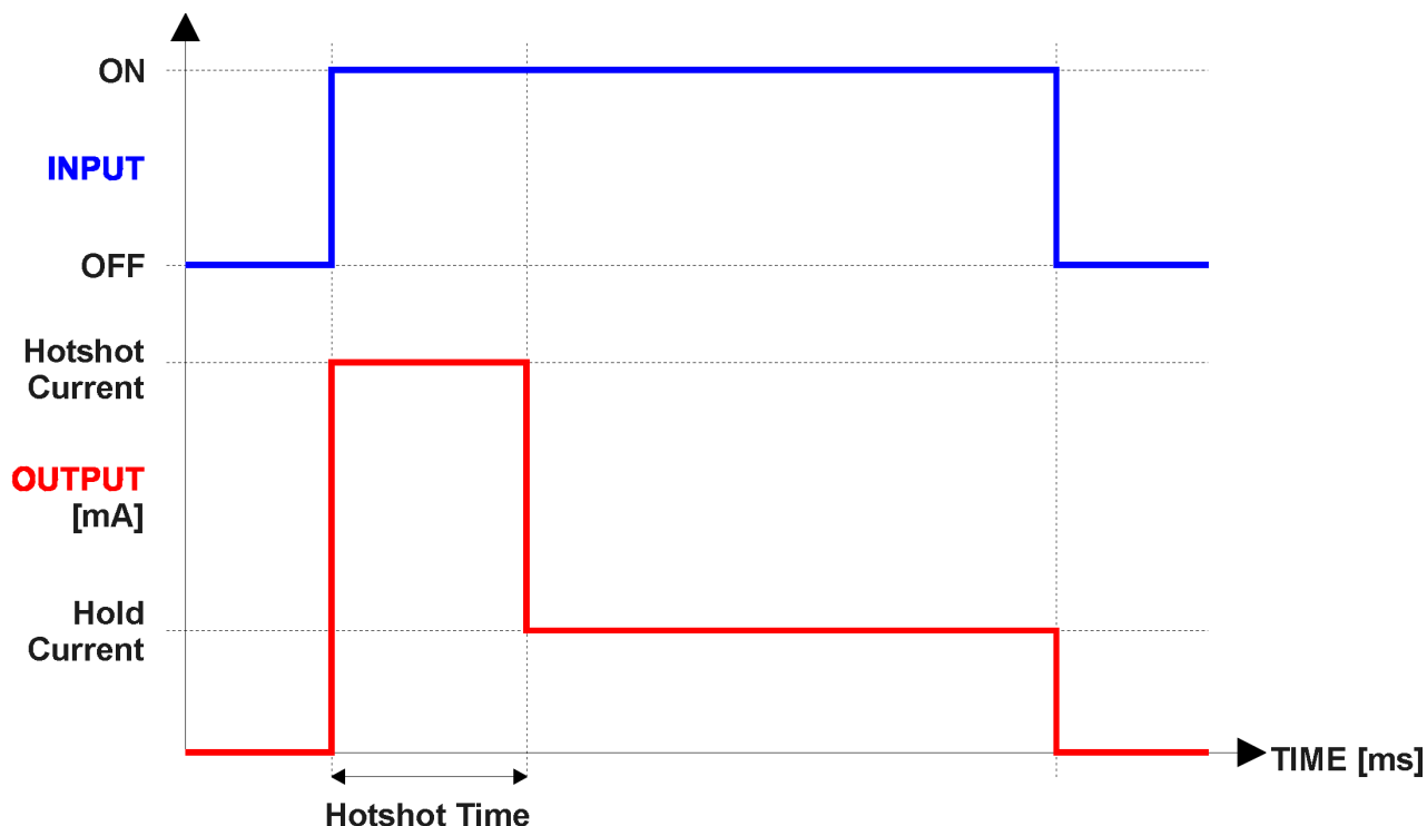
Figure 8 – Hotshot Digital Profile
