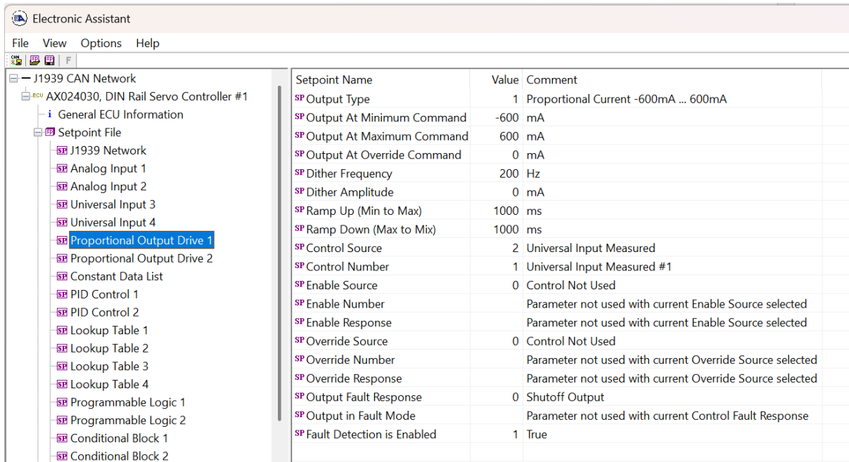
Figure 9 - Screen Capture of Proportional Output Setpoints
