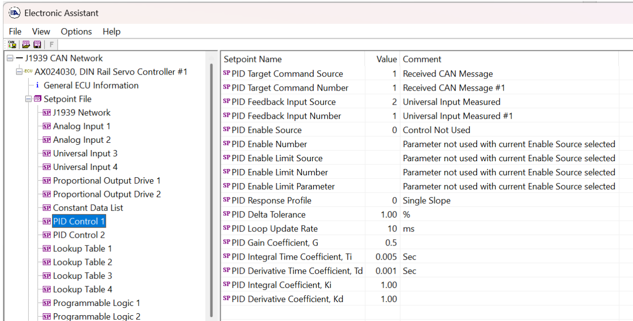
Figure 11 - Screen Capture of PID Control Setpoints
