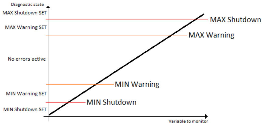
Figure 2 - Double Minimum and Maximum Error Thresholds
