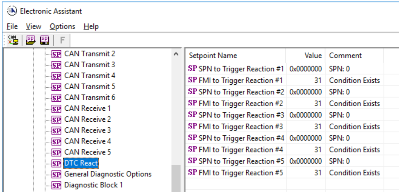
Figure 19 - Screen Capture of DTC React Setpoints
