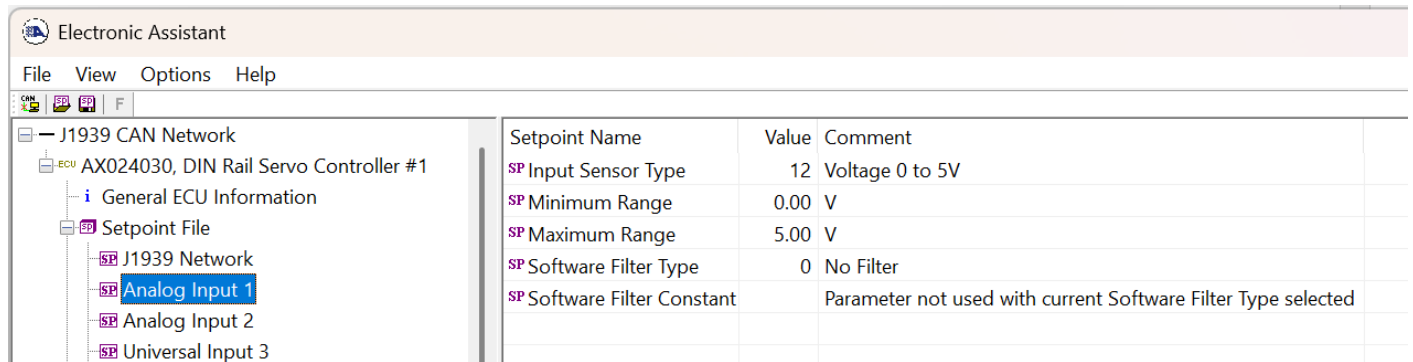
Figure 7 - Screen Capture of Analog Input Setpoints
