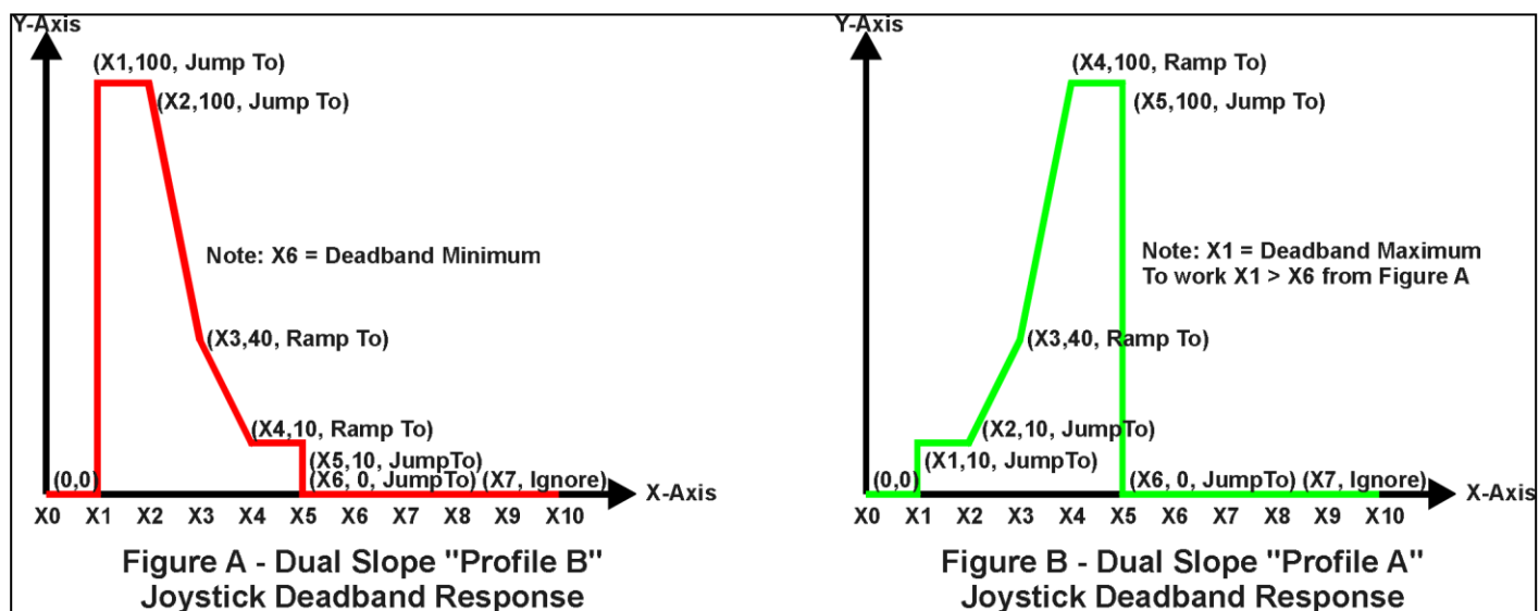
Figure 11 – Lookup Table Examples to Setup for Dual-Slope Joystick Deadband Response
