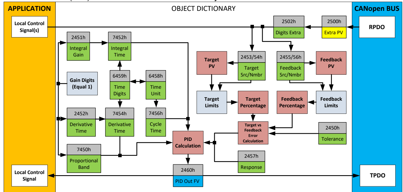
Figure 7 – PID Control Objects
