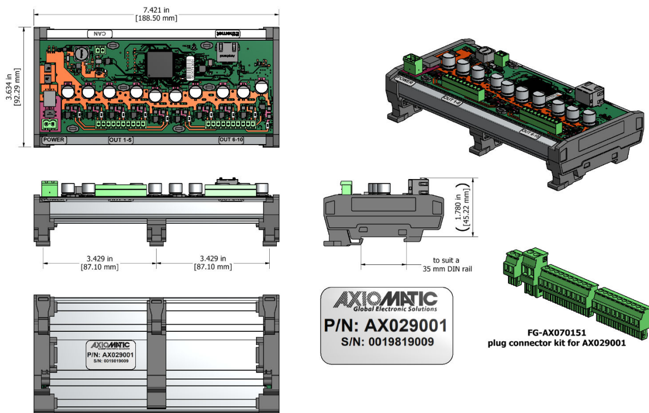
Figure 16 – Housing Dimensions
