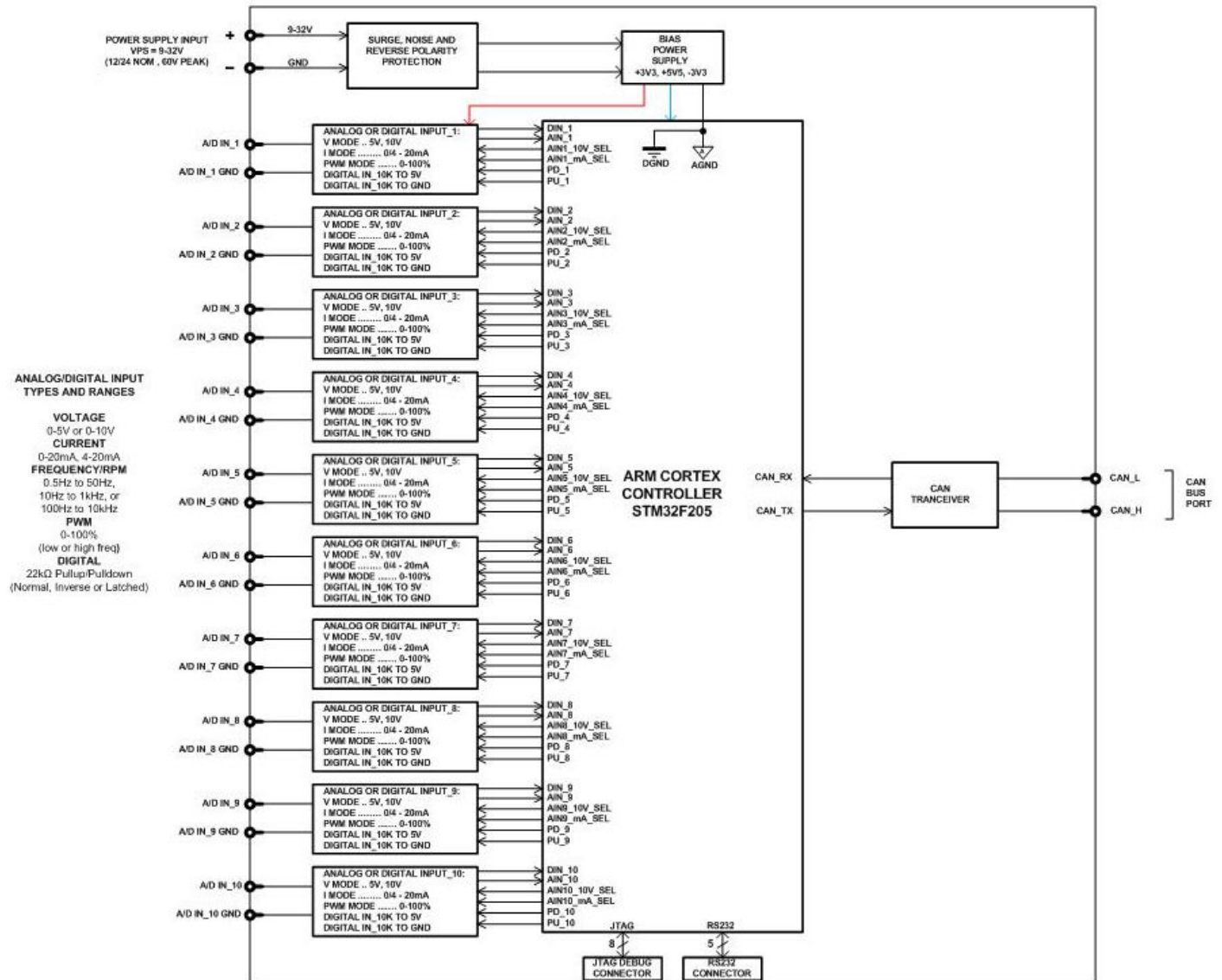
Figure 1A – Hardware Functional Block Diagram
