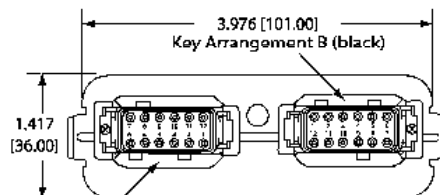
FRONT VIEW 24-PIN RECEPTACLE (NOT TO SCALE)
