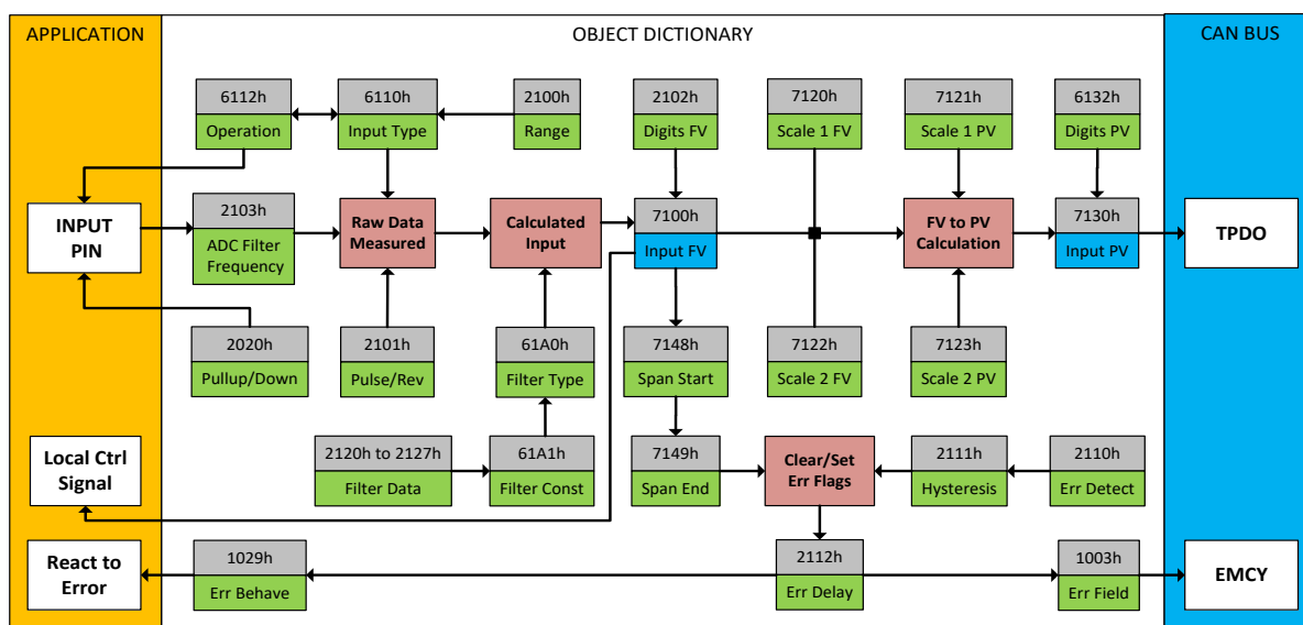
Figure 7 Analog Input Objects
