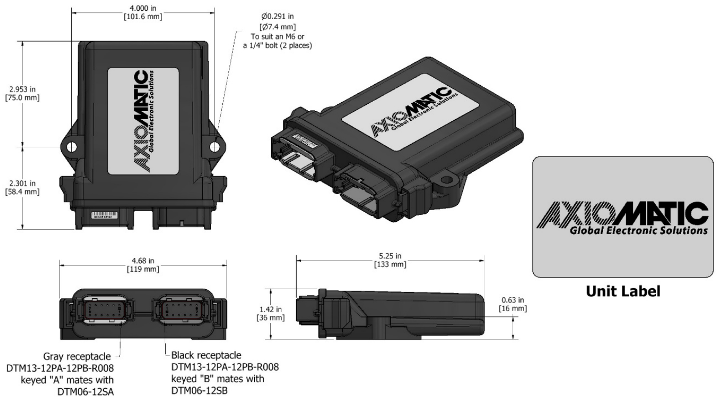
Figure 14 - Housing Dimensions
