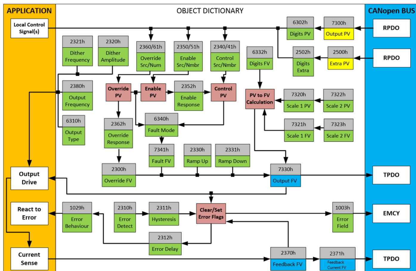
Figure 9 – Analog Output Objects
