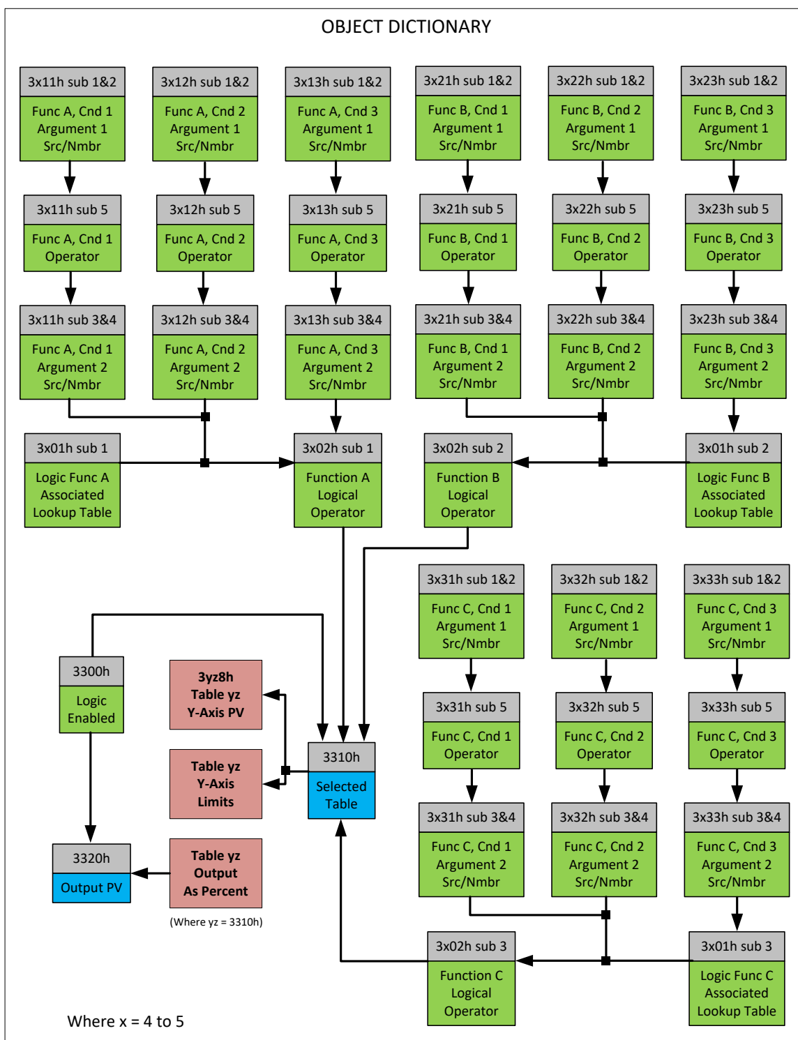
Figure 18 – Logic Block Objects
