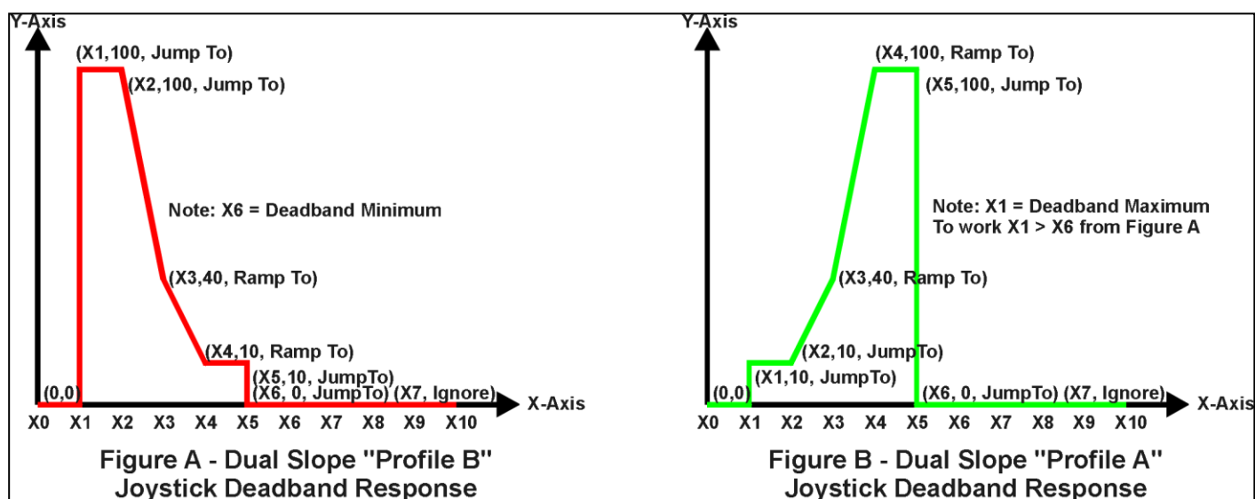
Figure 17 – Lookup Table Examples to Setup for Dual-Slope Joystick Deadband
