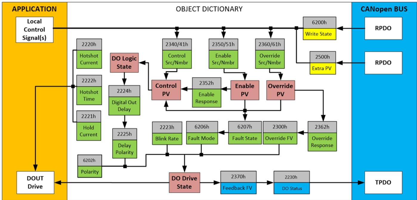
Figure 7 – Digital Output Objects
