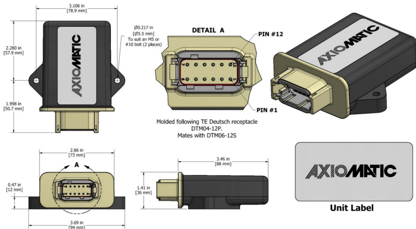
Figure 23 – Housing Dimensions
