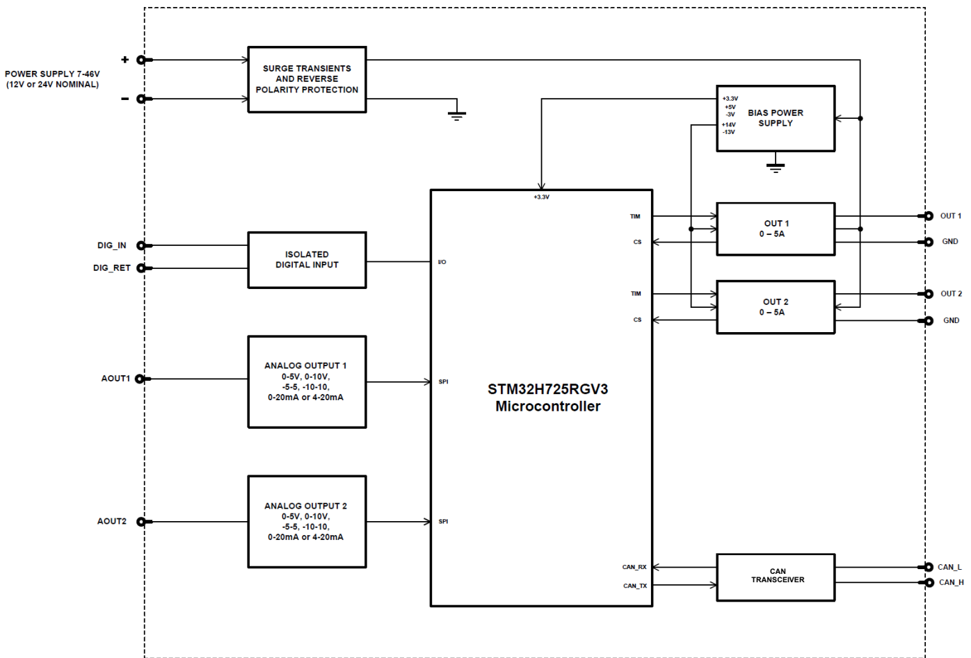
Figure 1 – Hardware Block Diagram
