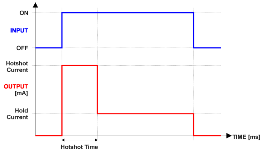
Figure 8 – Hotshot Digital Profile
