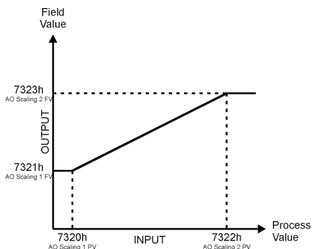
Figure 10 – Analog Output Linear Scaling PV to FV
