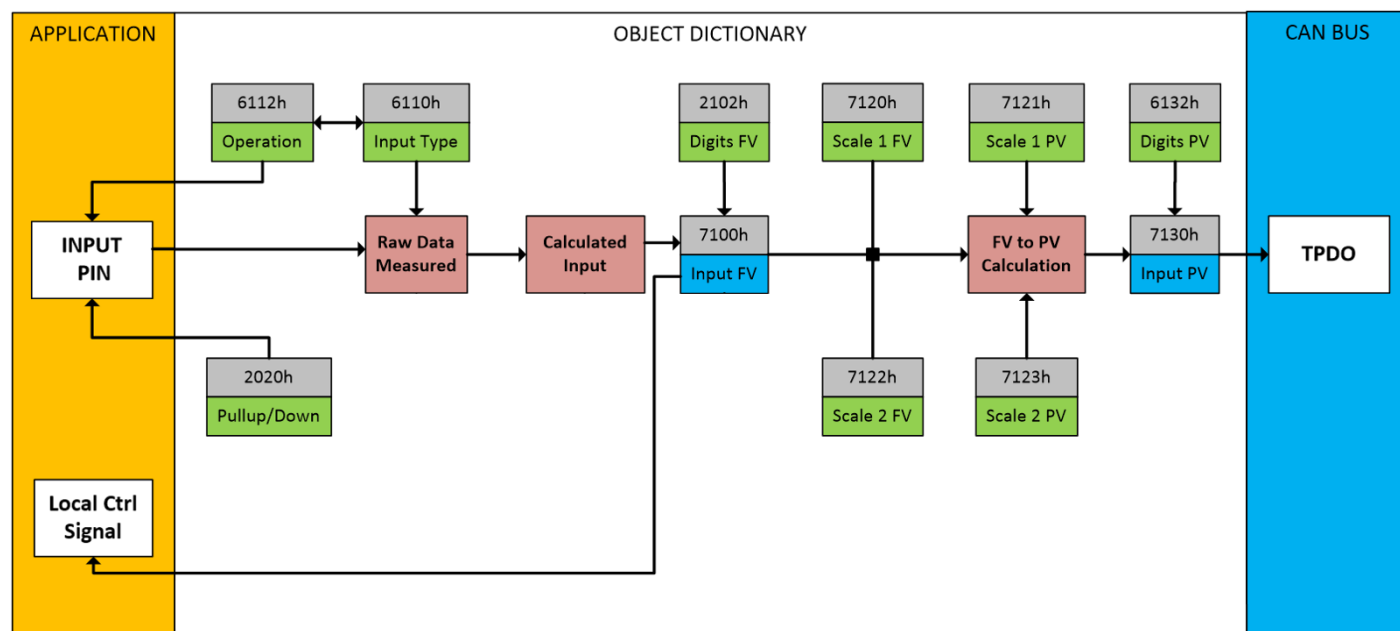
Figure 5 – Analog Input Objects
