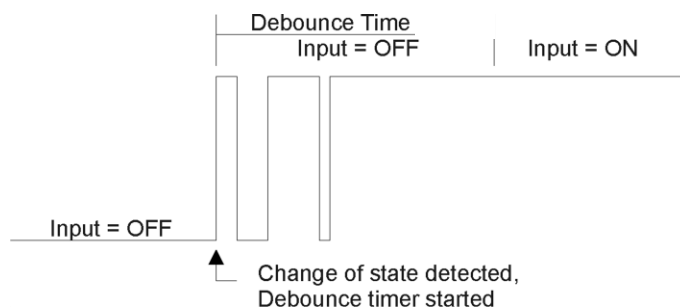
Figure 4 – Digital Input Debouncing
