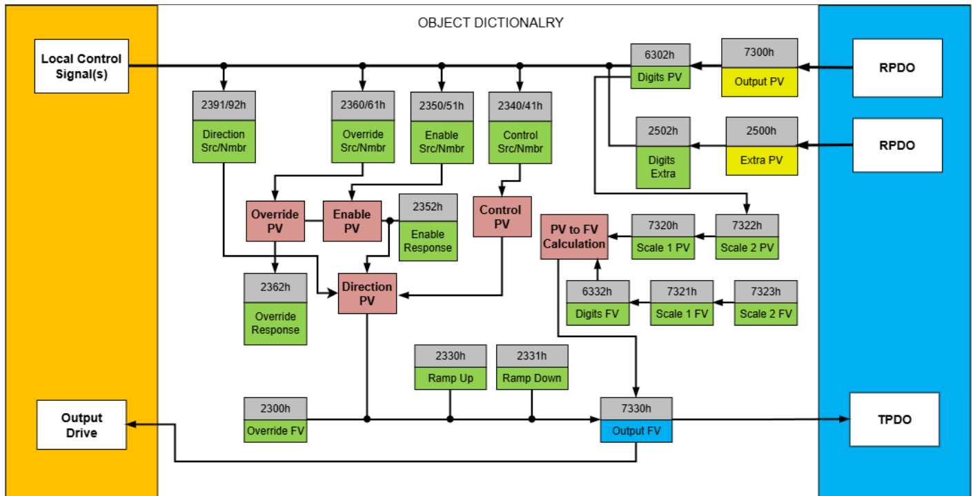
Figure 11 – H-Bridge Drive Objects
