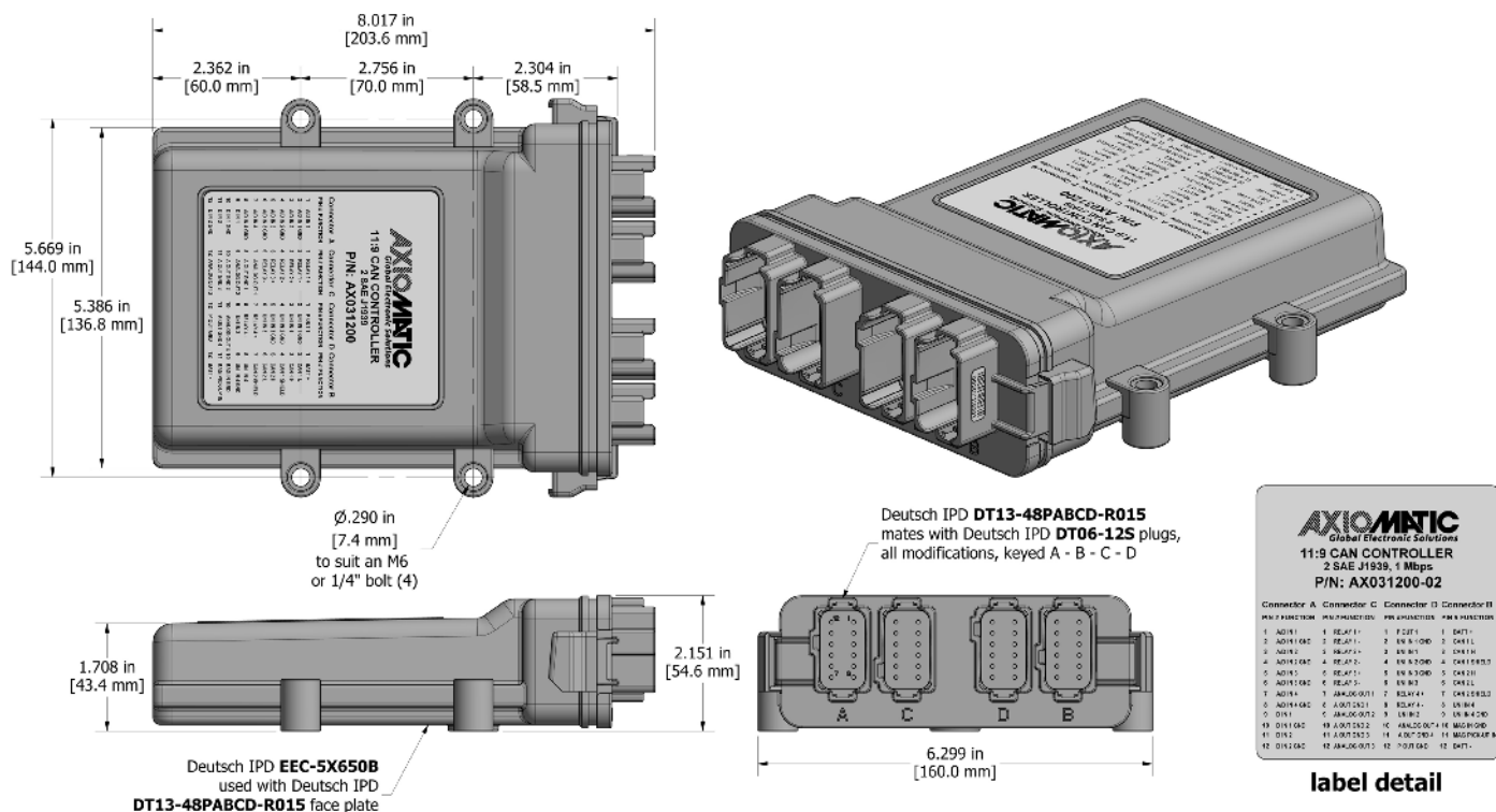
Figure 6 – AX031200 Dimensional Drawing
