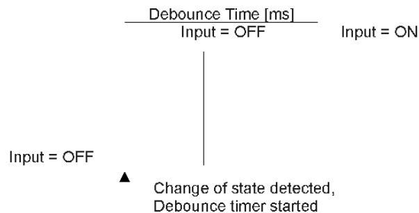
Figure 4 – Input Debouncing
