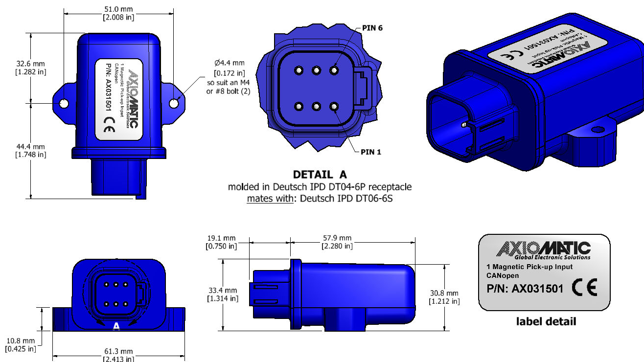
Figure 14 – AX031501 Housing Dimensions
