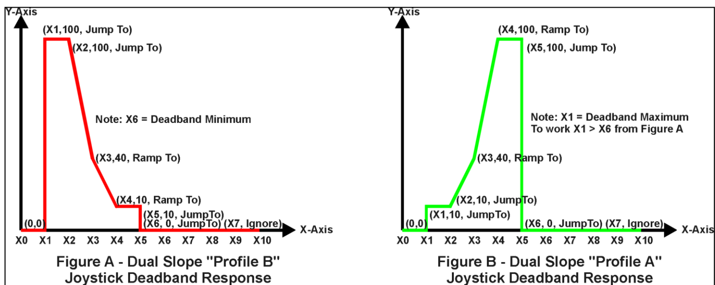
Figure 12 – Lookup Table Examples to Setup for Dual-Slope Joystick Deadband Response
