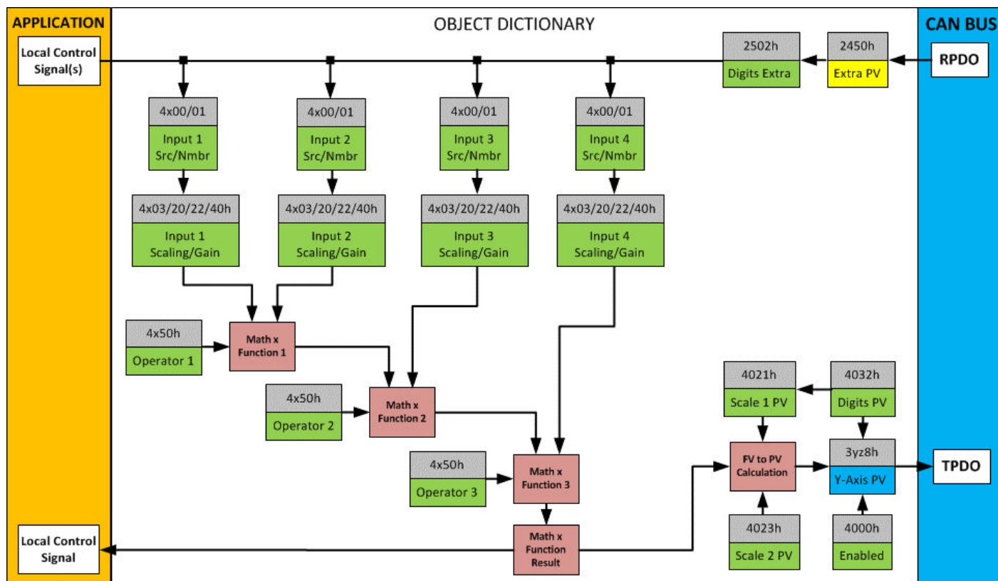
Figure 15 – Math Function Block Objects
