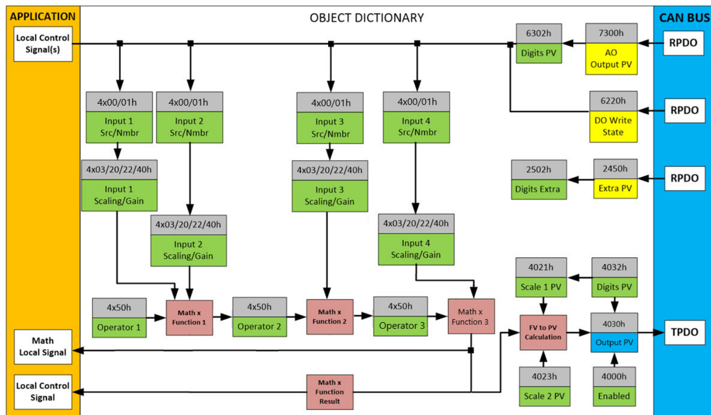
Figure 13 - Math Function Block Objects
