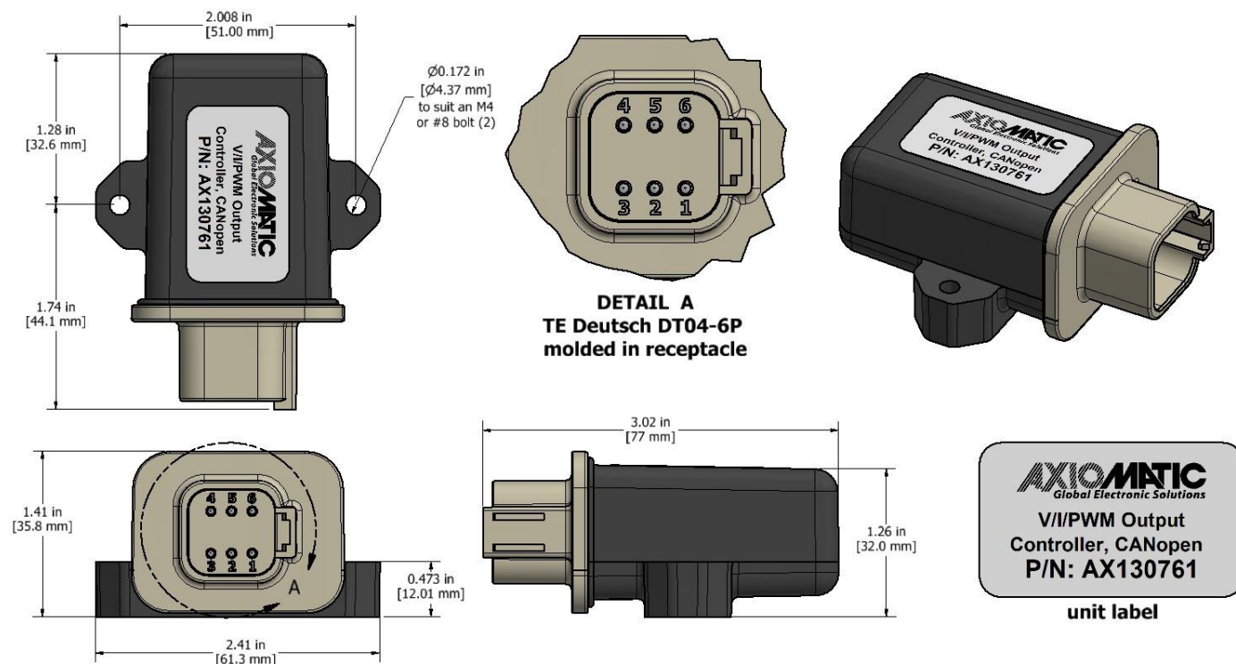
Figure 16 - Housing Dimensions
