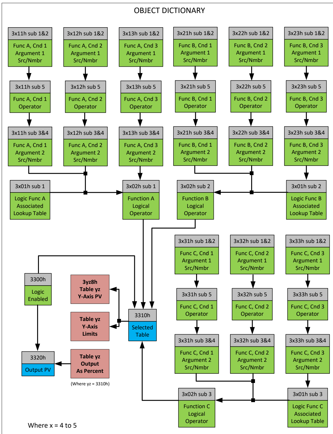
Figure 11 - Logic Block Objects
