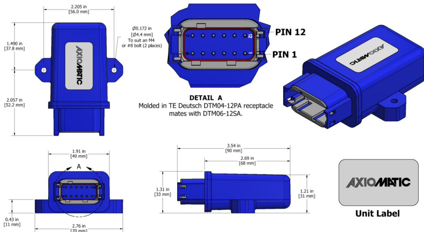
Figure 23 – Housing Dimensions
