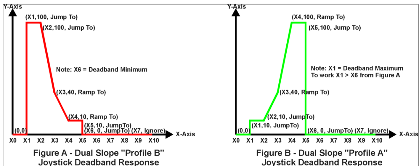
Figure 17 – Lookup Table Examples to Setup for Dual-Slope Joystick Deadband
