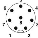
Schematic diagram pin assignment M12 plug, 8-positions, A-coded
