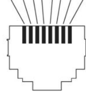
Schematic diagram connector pin assignment RJ45 plug
